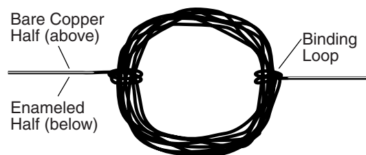
Figure 2. Coil Armature
