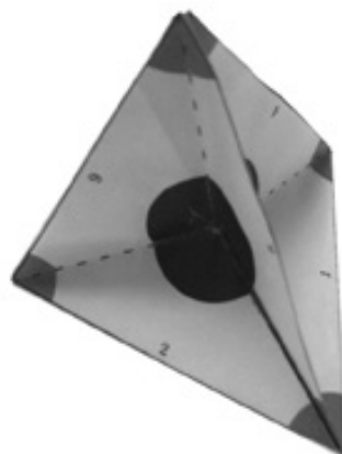
Tetrahedral
