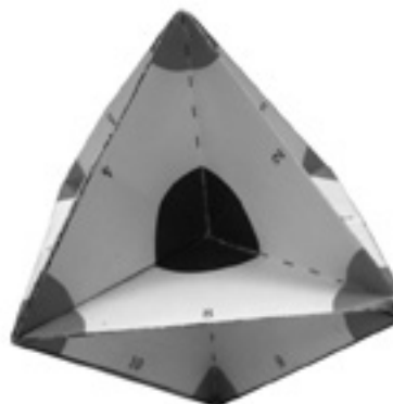
Octahedral
