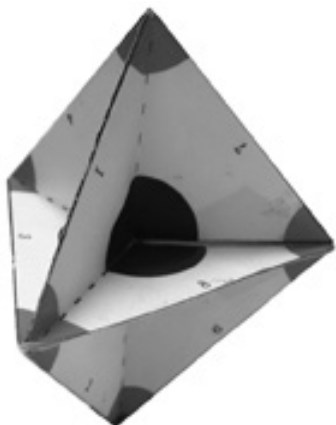
Trigonal Bipyramidal
