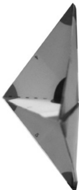
Seesaw
